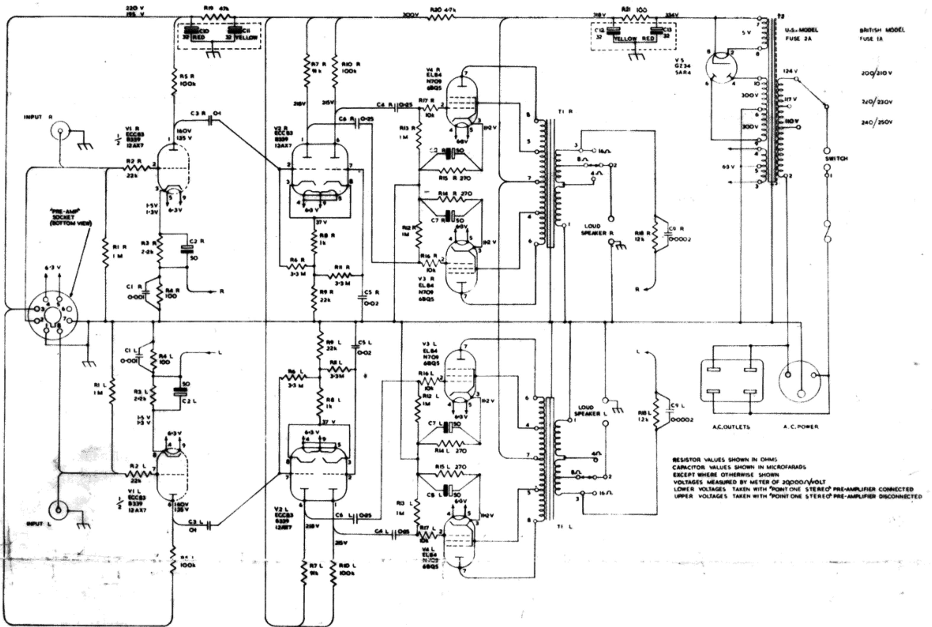
CIRCUIT DIAGRAM
