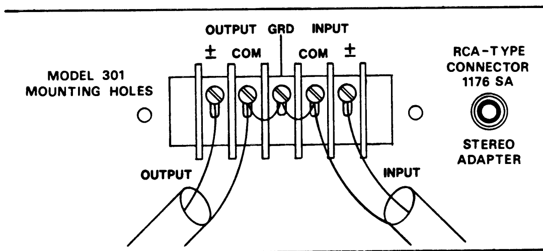
FIGURE 2-2. CONNECTING THE MODEL 1176LN WITH UNBALANCED INPUT AND UNBALANCED OUTPUT CIRCUITS.*
