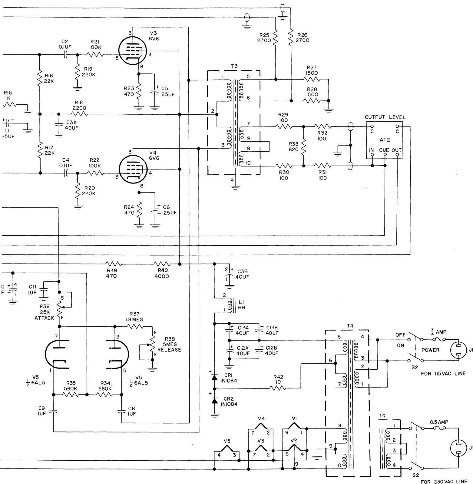
Figure 7-1. Peak Limiting Amplifier 26U-1, Schematic Diagram
