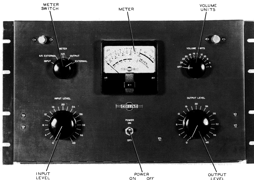
Figure 3-1. Operation Controls
