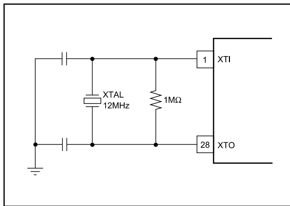
FIGURE 2. 12MHz Crystal Resonator Connection.
