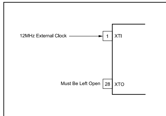
FIGURE 3. External 12MHz Clock Input Connection.
