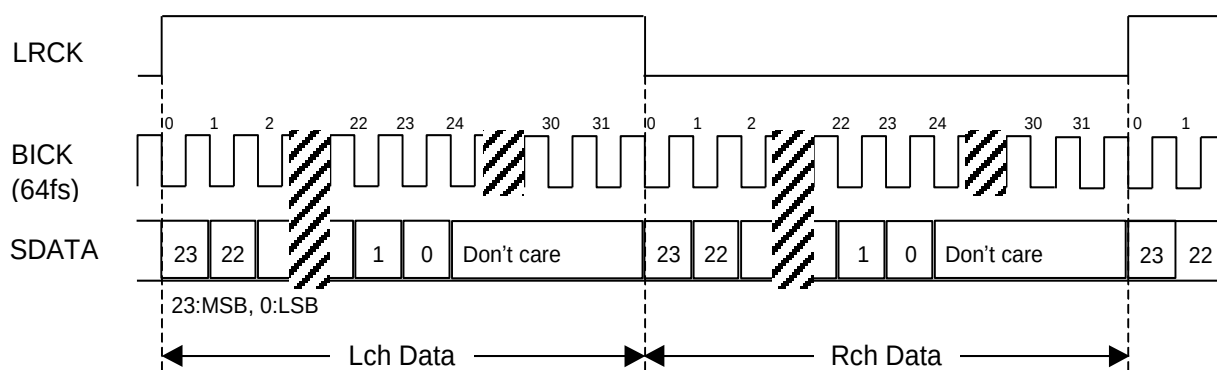
Figure 13. Mode 2 Timing
