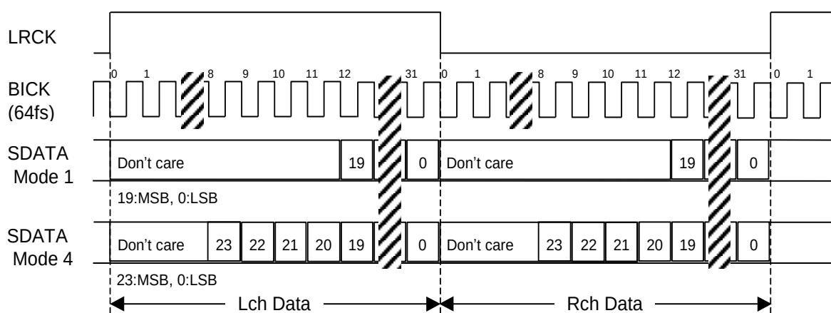
Figure 12. Mode 1/4 Timing
