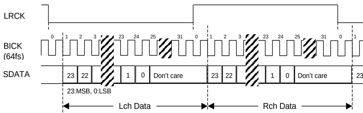
Figure 14. Mode 3 Timing
