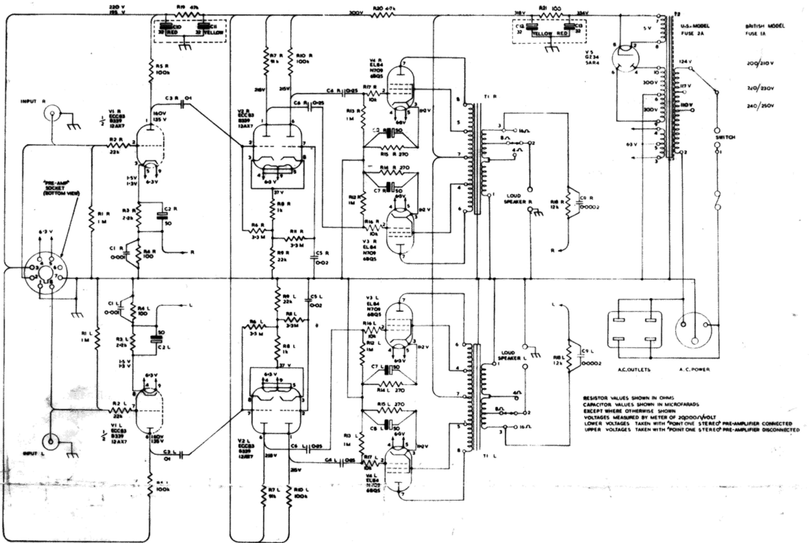
CIRCUIT DIAGRAM
