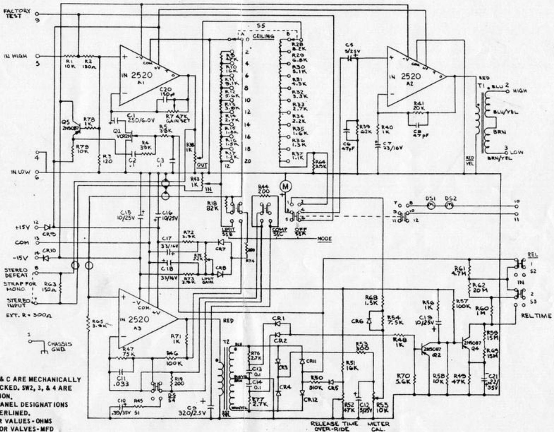
MODEL 525C AUDIO COMPRESSOR-LIMITER
